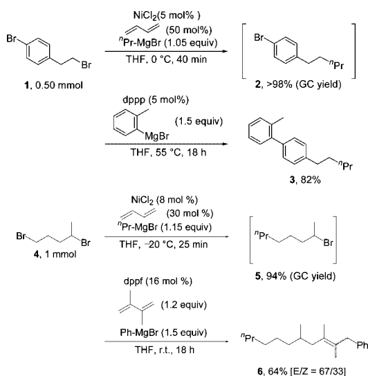
SCHEME 6. Site-Selective Sequential Cross-Coupling Using Unsymmetrical Dibromides
